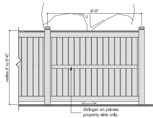
2 Solid Fence Elevation - Typ. 1BW Solid Fence Design - NTS
