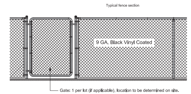
5 Rear Yard Chain-link Fence Elevation - Typ. 1BW Chain-link Fence Design - NTS
