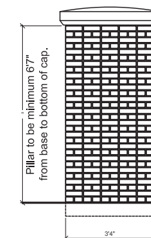
8 Pillar Elevation - Typ. 1BW Roundabout Pillar Design - NTS
