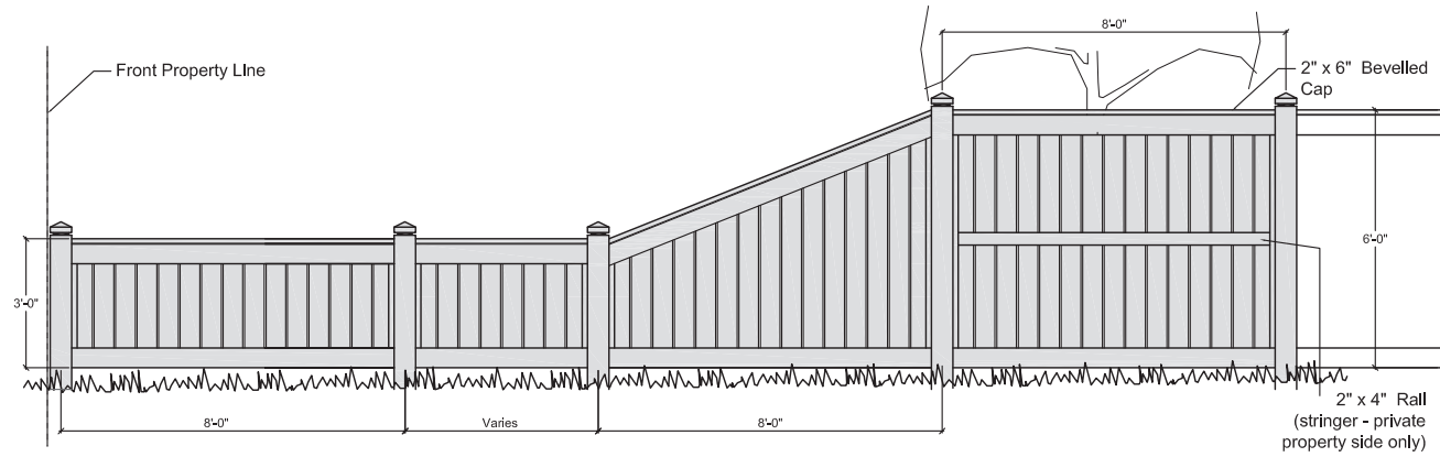
1 Solid Wood Fence - Street or Path Side Yard - Typ. 1BW Solid Wood Fence Design - NTS
