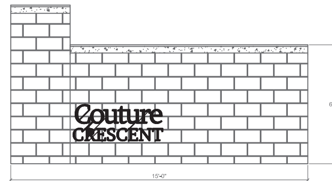
7 Minor Entry Detail facing Couture Crescent - Typ. 1BW Masonry Fence - NTS
