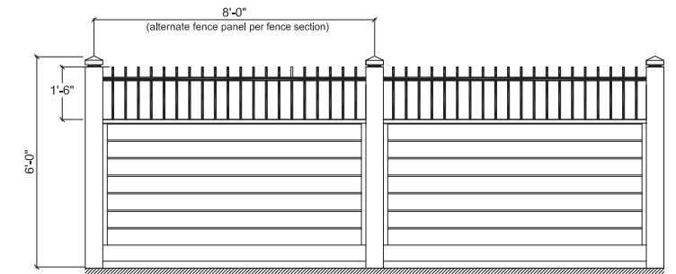
3 Solid Fence with Wrought Iron Top - Typ. 1BW Solid Fence with Wrought Iron Top - NTS
